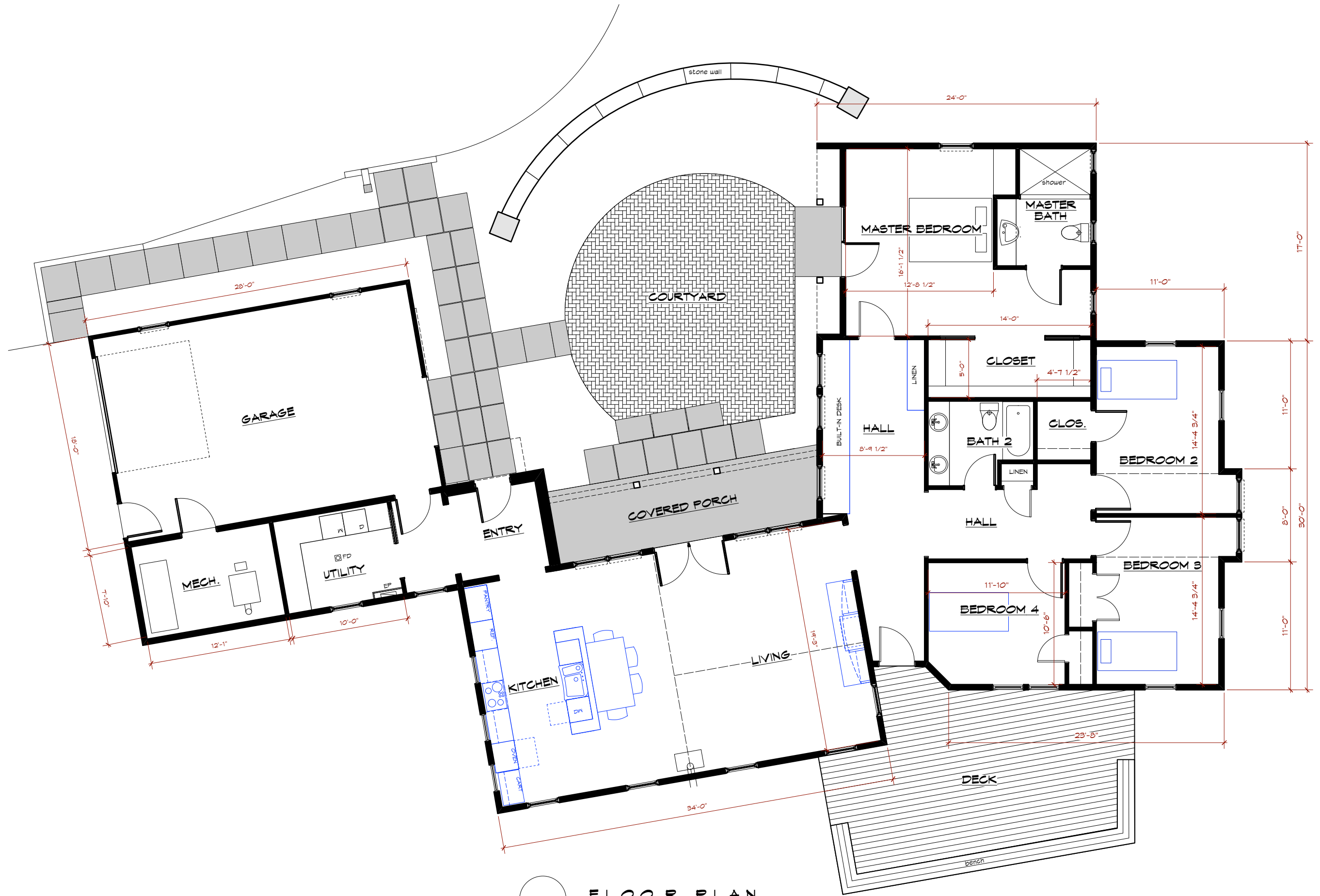
FLOOR PLAN 2370 sf
