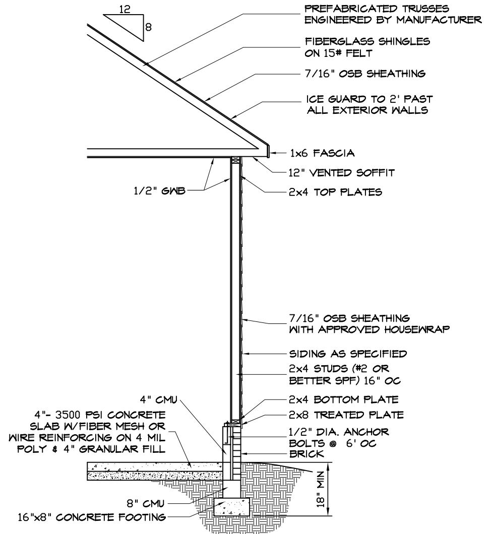
GARAGE WALL SECTION (TYP.)
