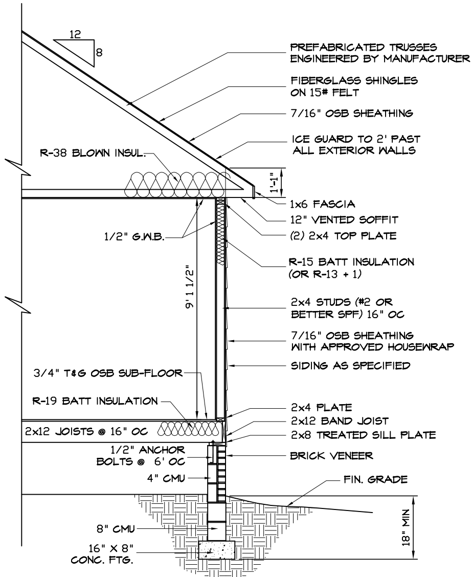
WALL SECTION (TYP.)
