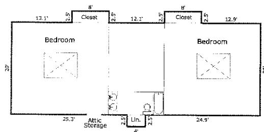
SECOND FLOOR - 1,055 SF
