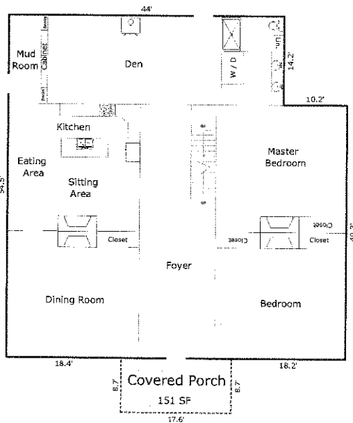
MAIN FLOOR - 2,809 SF
