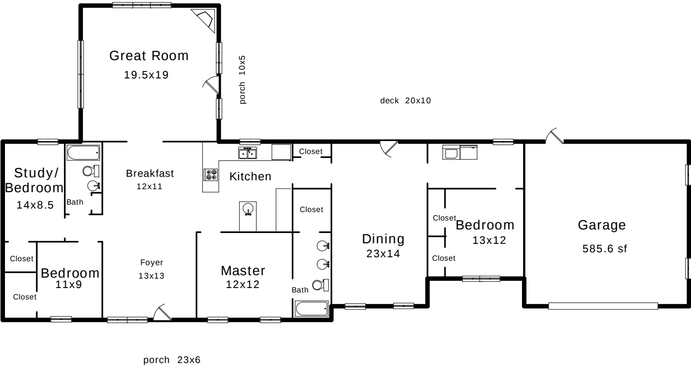
Main House 2295.5 sf
