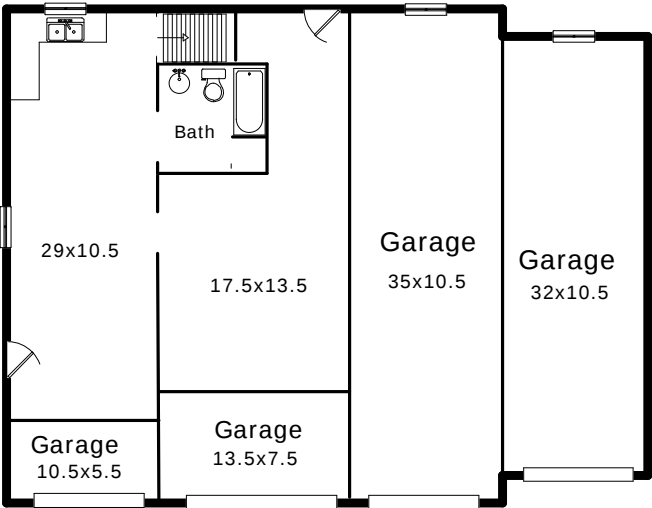
Guest House Main Floor 747 sq ft
