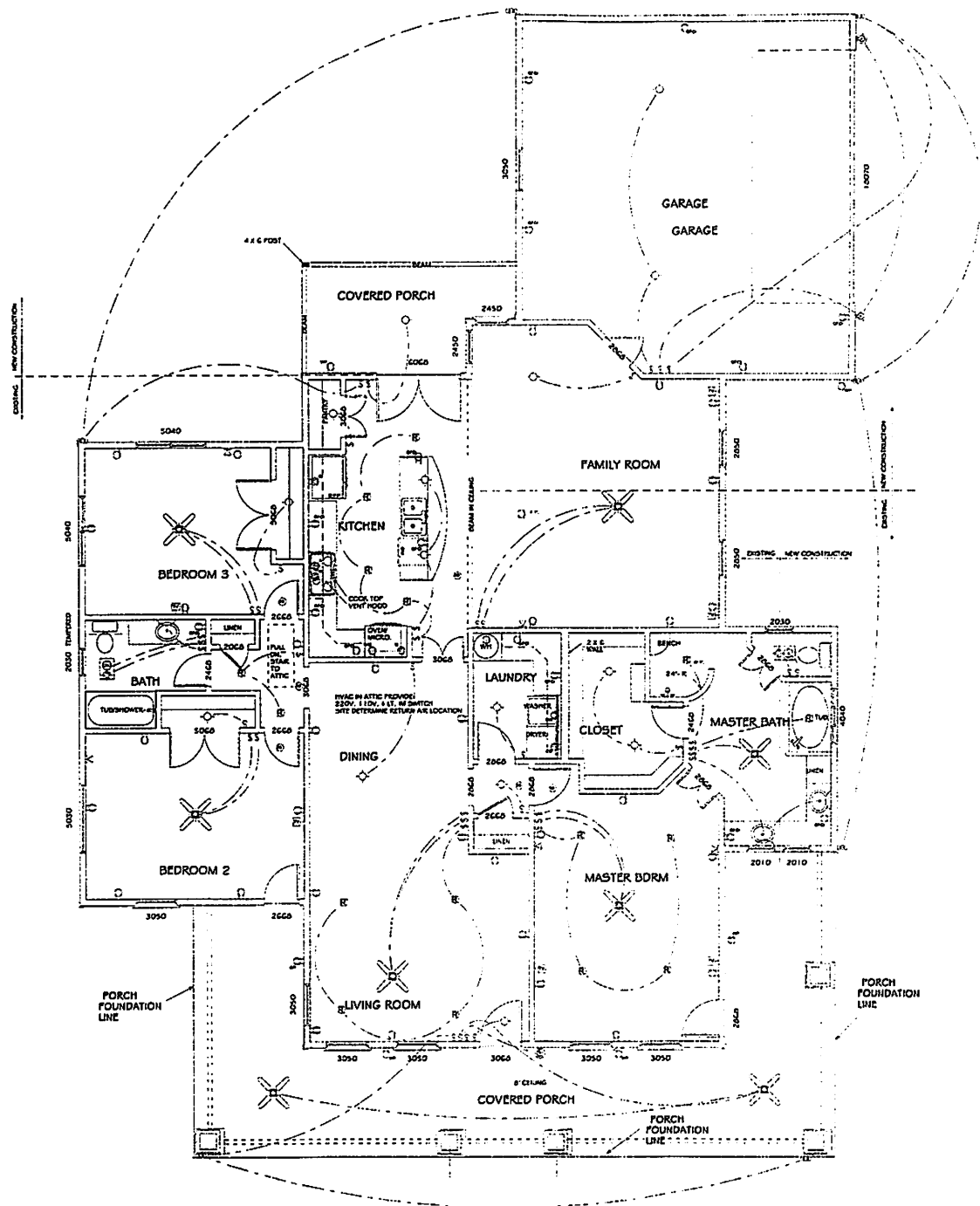
1/4" = 1'-0"
