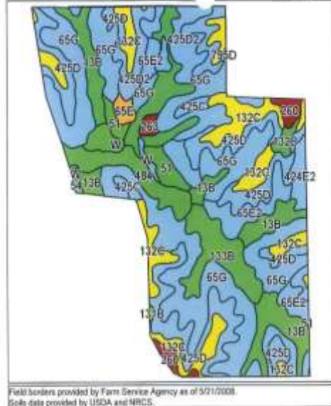
Soils Map
