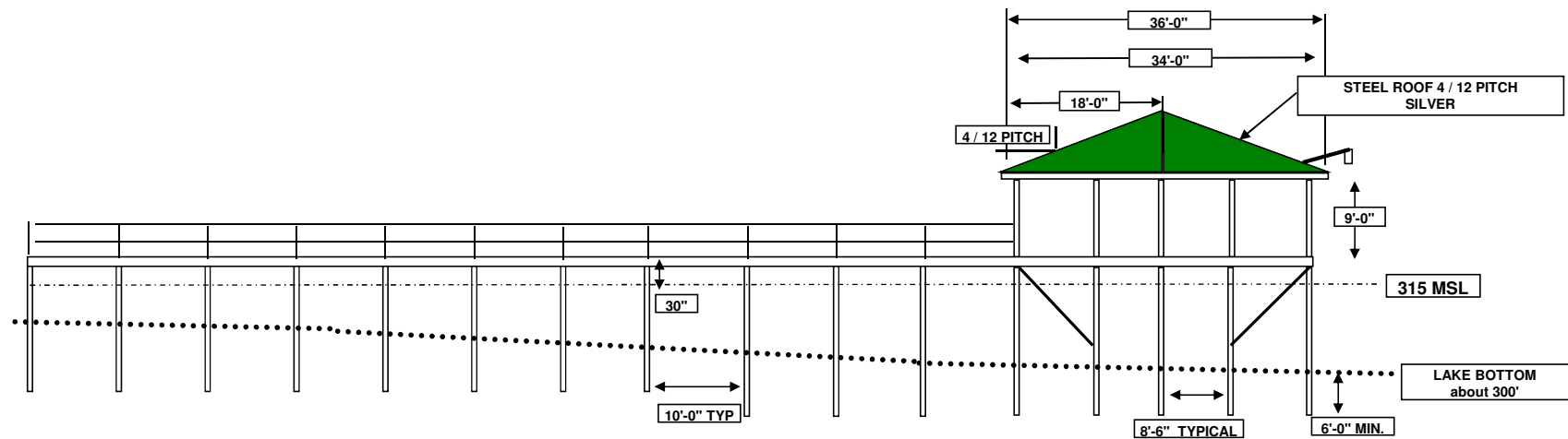
RIGHT SIDE VIEW
