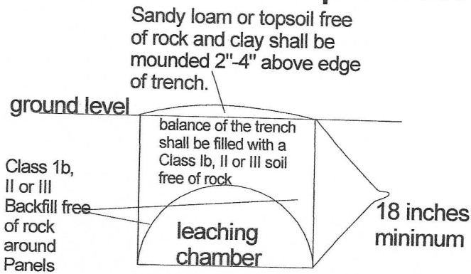
3' Cross Section of Trench using leaching chambers
