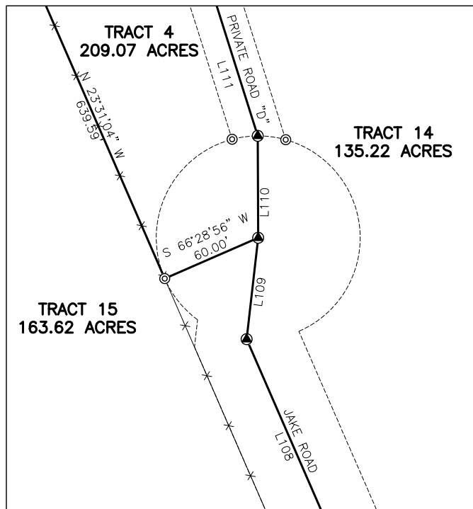
DETAIL No. 5 SCALE 1"=80'
