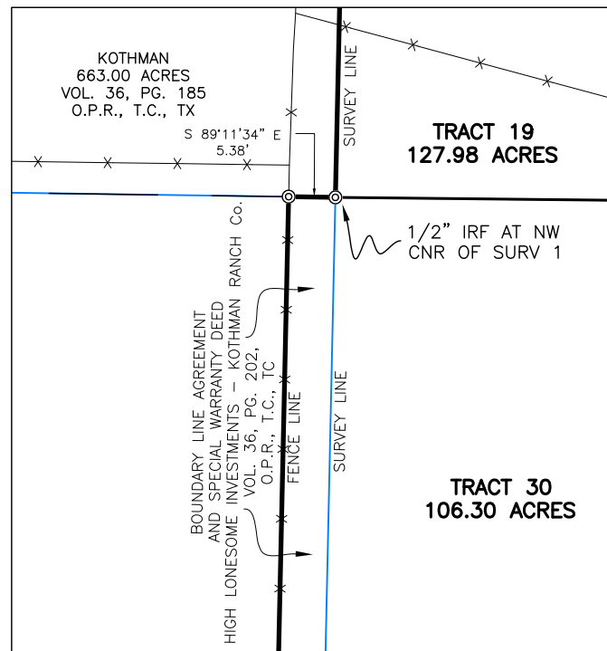
DETAIL No. 4 SCALE 1"=20'
