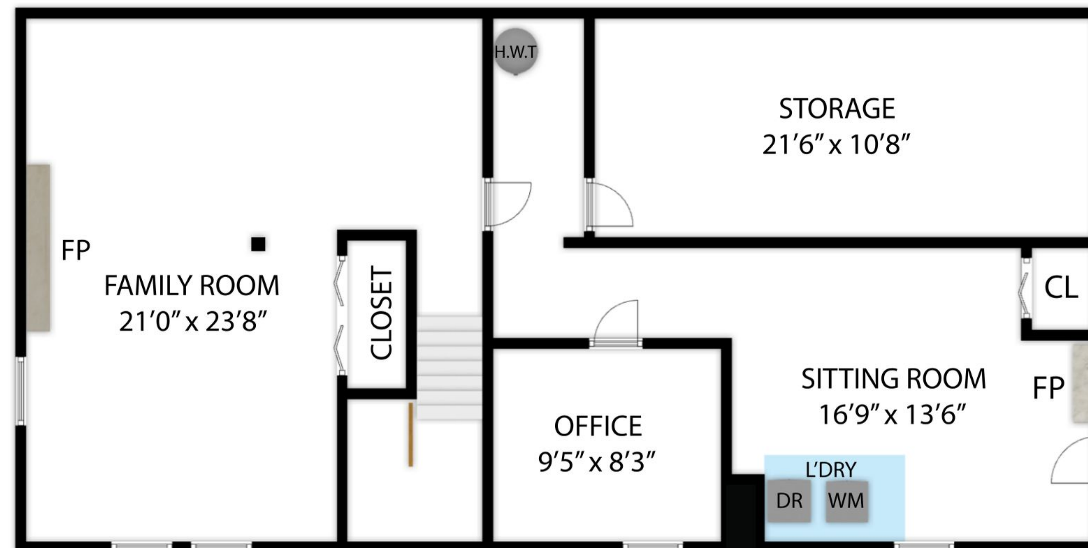
BASEMENT
