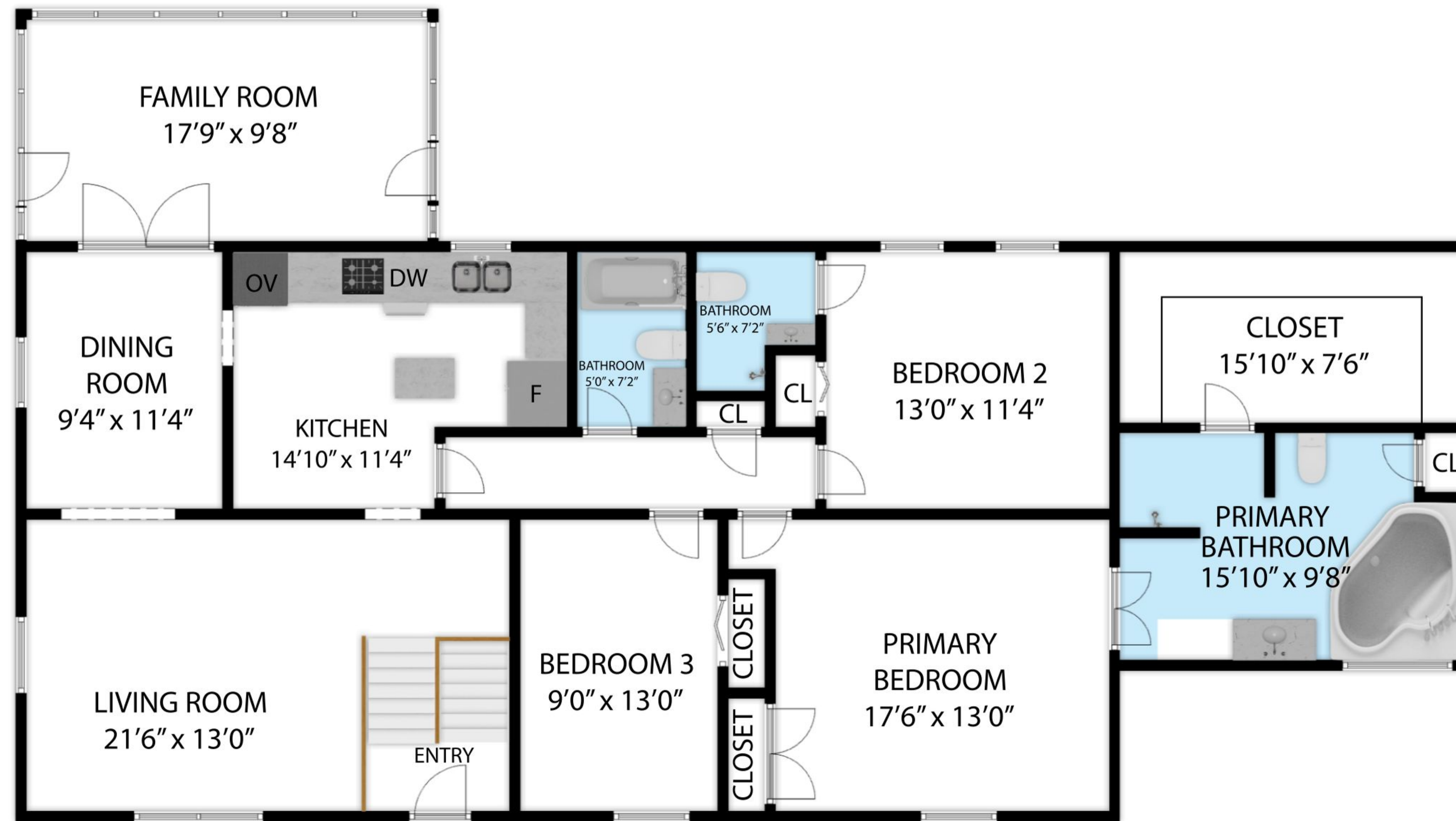
FIRST FLOOR
