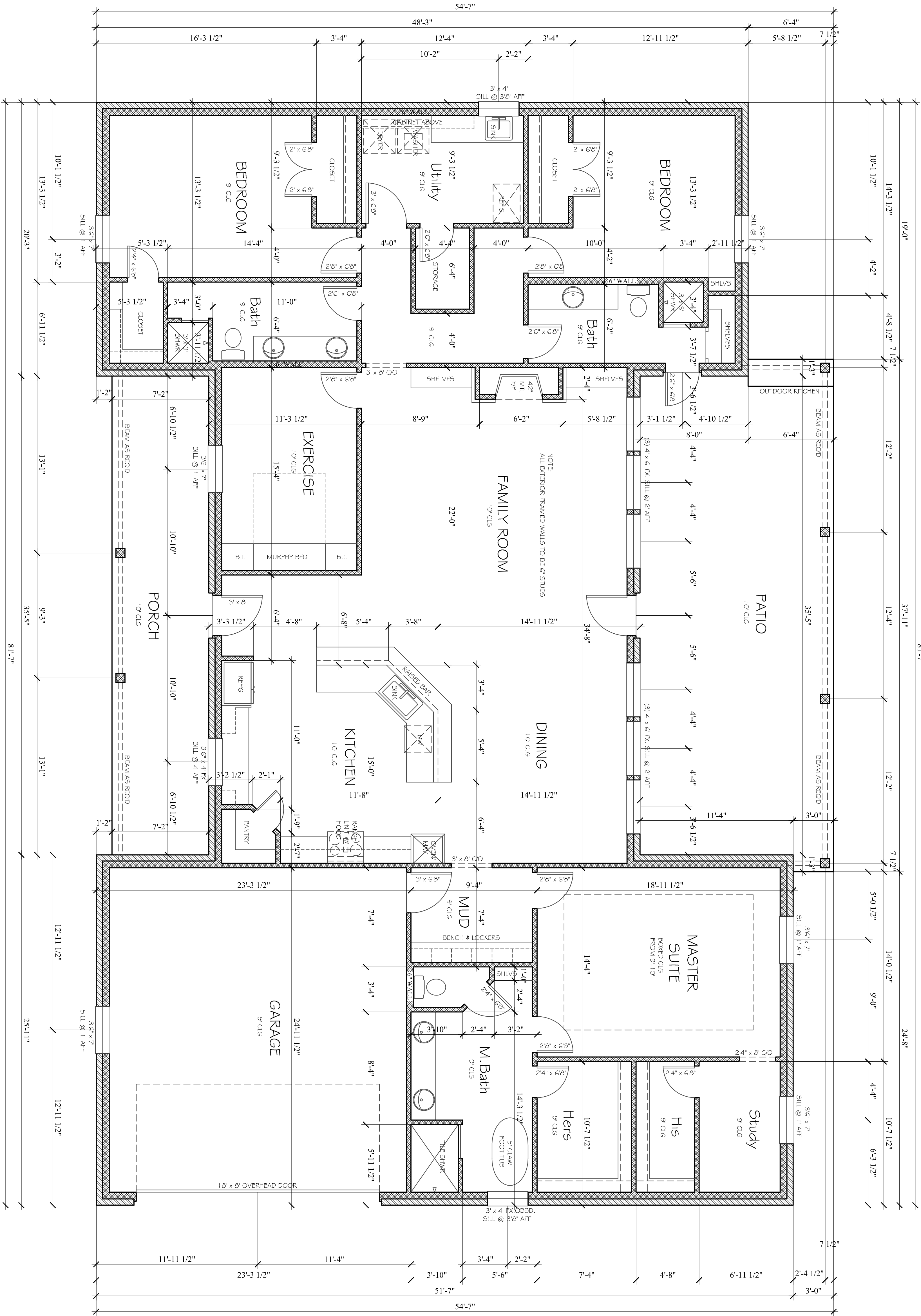
FLOOR PLAN
