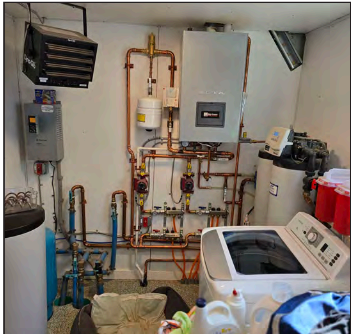
Mechanical Room
