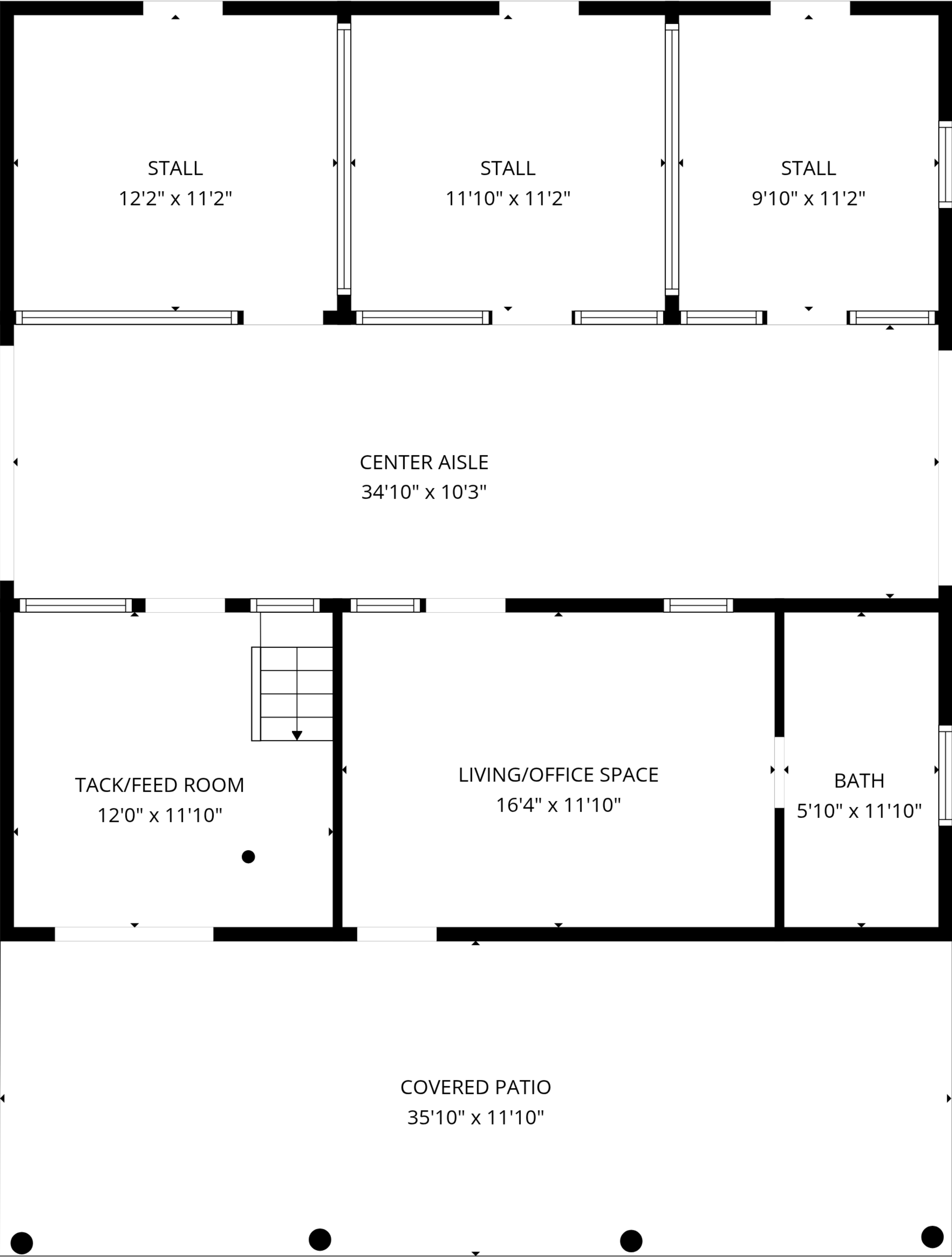
FLOOR 1
